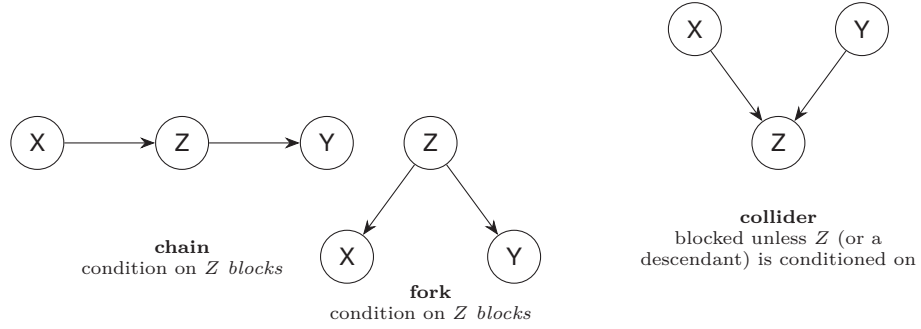
Figure A.1: The three path configurations behind d-separation (Definitions A.3.18 and A.3.20): chains and forks are non-colliders (conditioning on the middle node blocks the path); a collider blocks the path by default and is opened by conditioning on it or any of its descendants.
