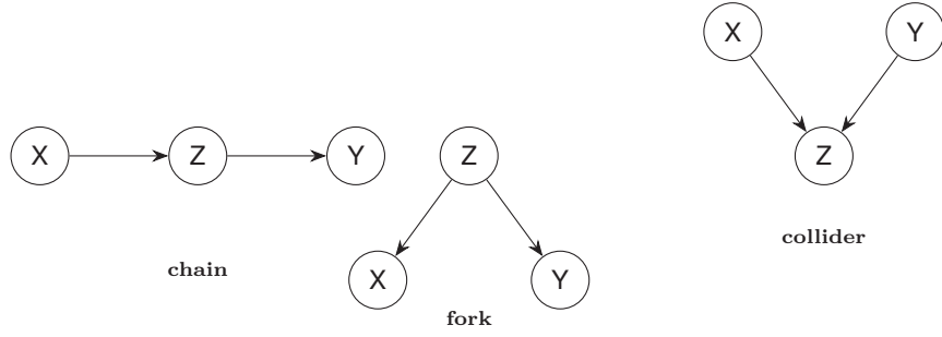
Figure A.2: The three local directed configurations of Definition A.4.6. The middle node is a non-collider in a chain or fork and a collider in the final configuration.
