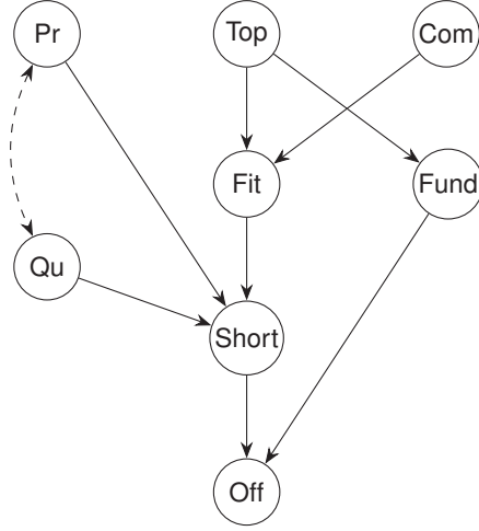
Figure A.1: The observed graph of Figure 5.3, now as directed and bidirected packages. The dashed edge is the latent U_B of the SCM drawing, inducing \text{Pr} \leftrightarrow \text{Qu} .
