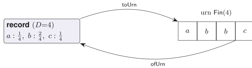
Figure 5.1: Record and urn presentations of a finite rational distribution agree on every decidable event (Proposition B.6.11); the maps toUrn / ofUrn are the computable witnesses checked in Lean.
