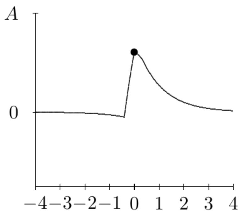
Figure 10.14: This is t = .4 .
