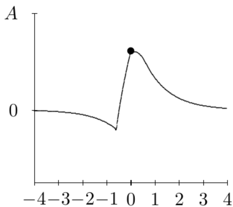
Figure 10.15: This is t = .6 .
