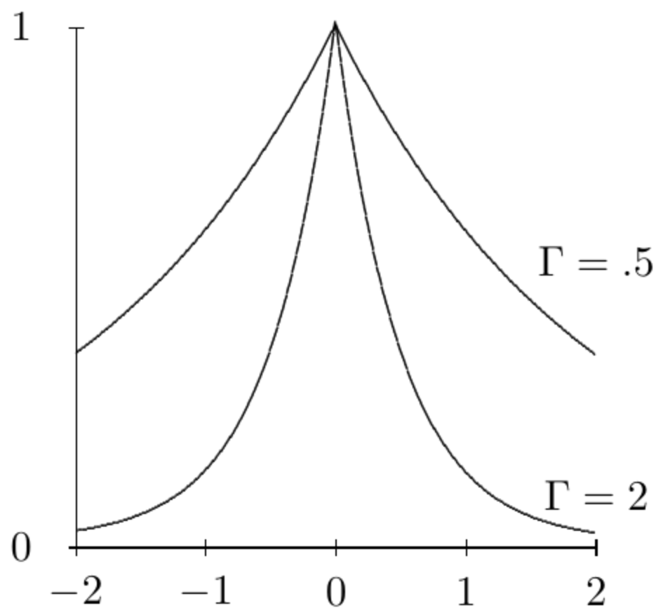
Figure 10.4: f(t) = e^{-|\Gamma t|} for \Gamma = 0.5 and \Gamma = 2 .
