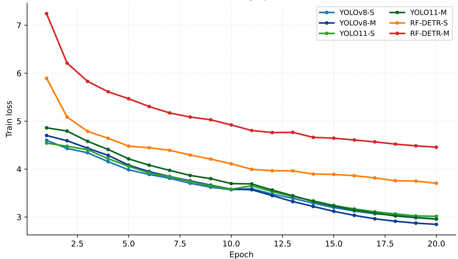
Train loss by epoch
