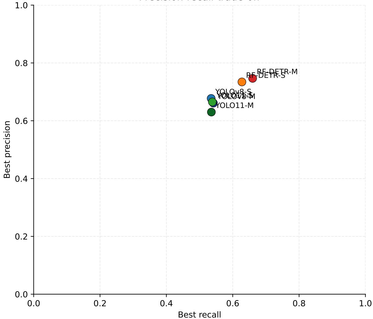
Precision-recall trade-off
