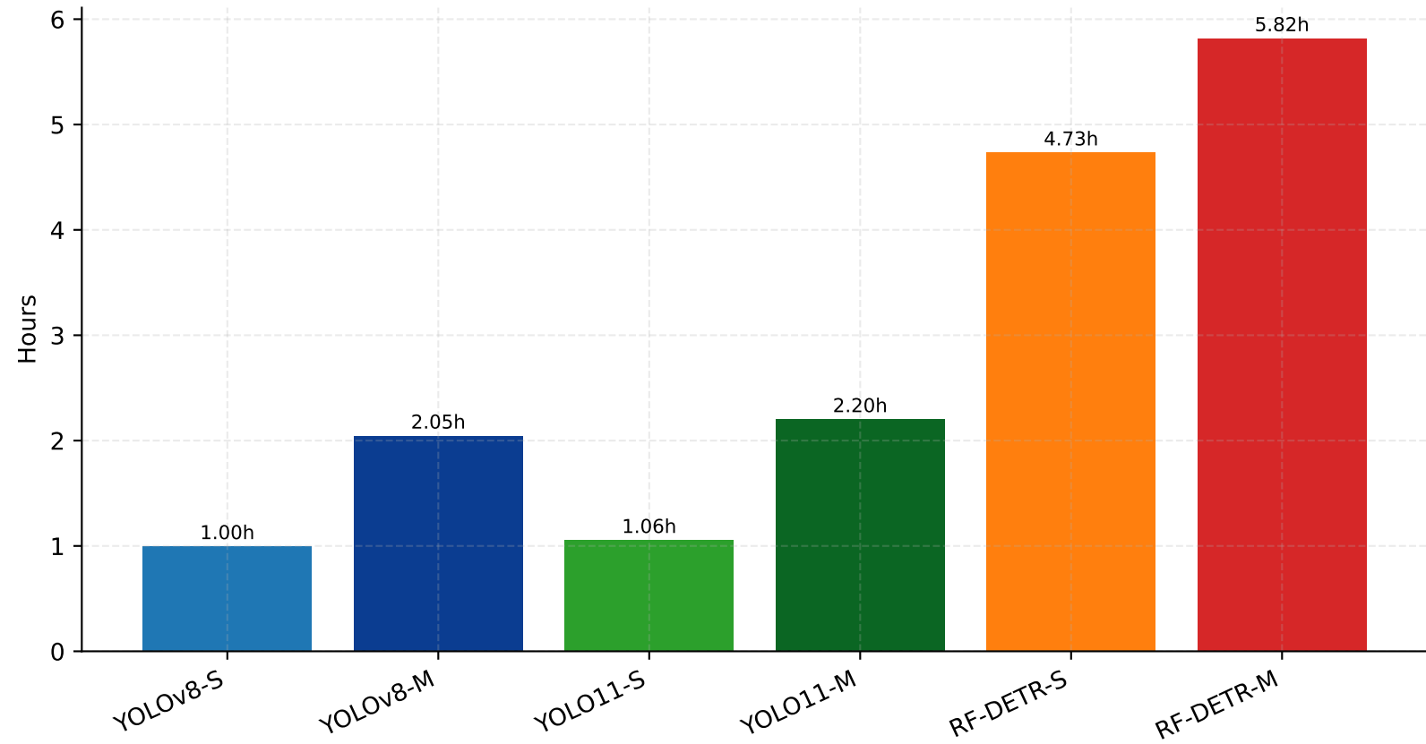
Training time
