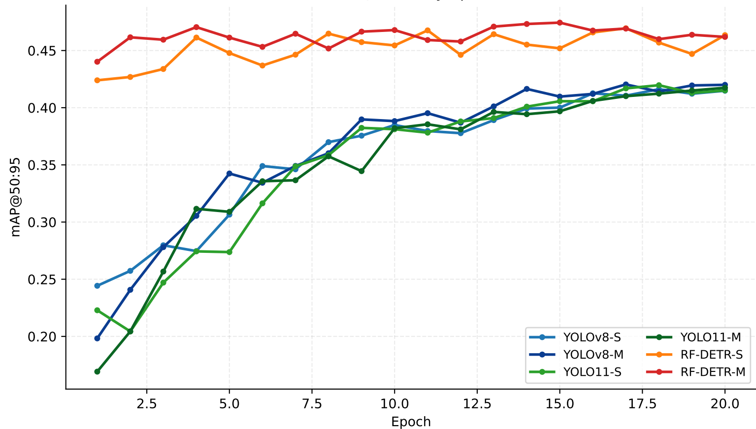
mAP@50:95 by epoch
