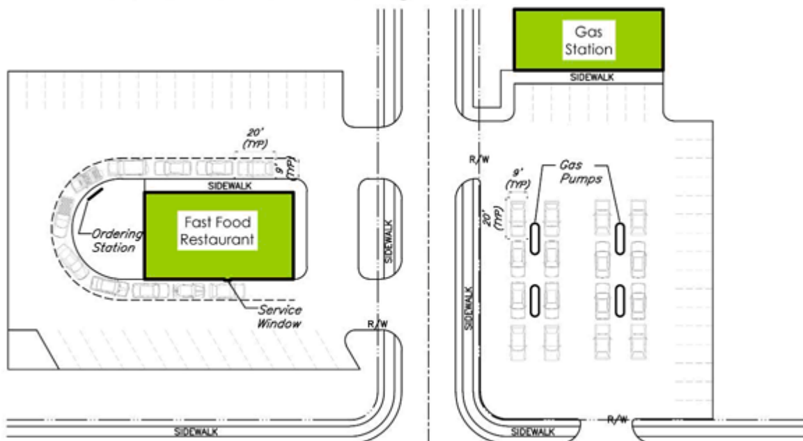
Figure 8-3, Drive Thru & Gas Station Stacking Requirements
