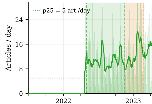
News volume
