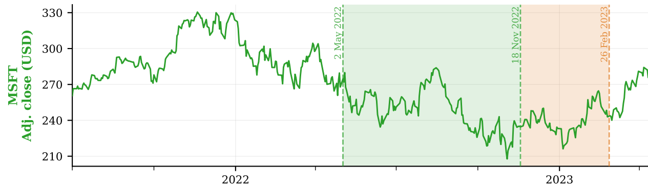
Price history
