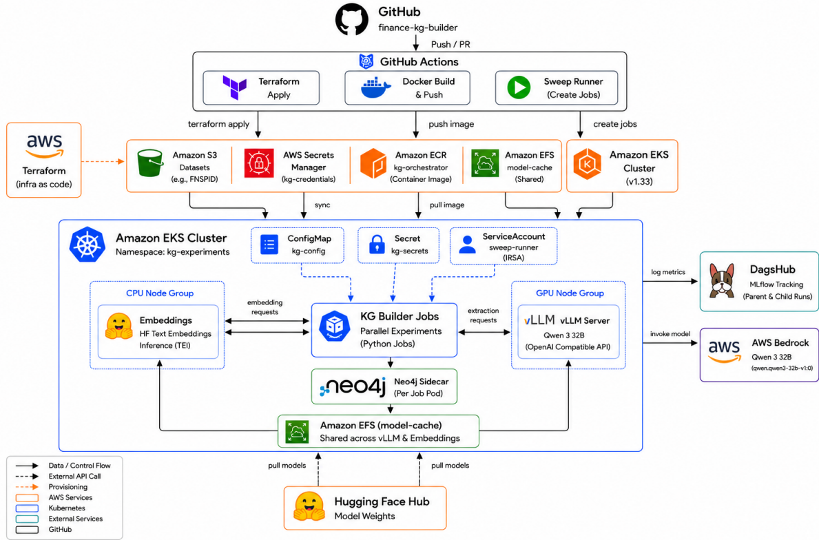
Figure 4: Experimental infrastructure.
