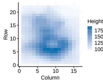
Volcano height heatmap
