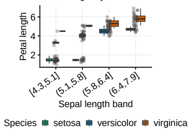
Petal length by size band
