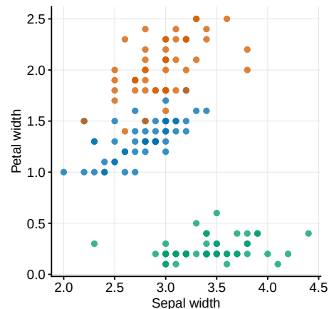
Fixed aspect scatter
