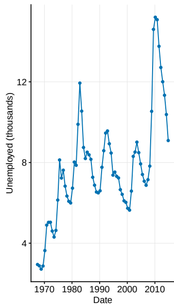
Unemployment over time
