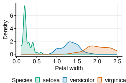
Petal width density
