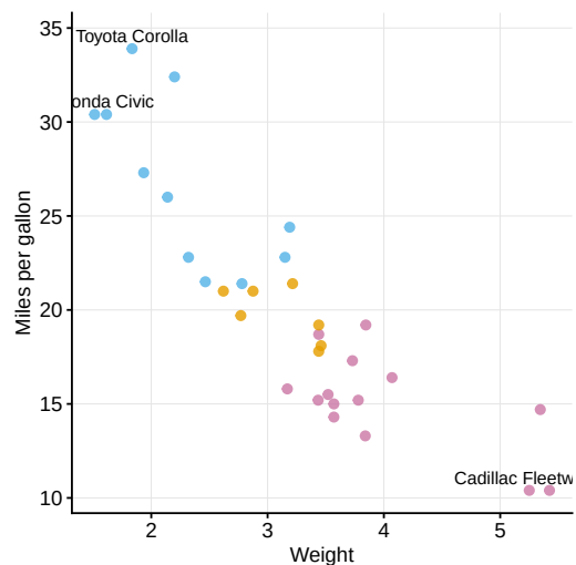
Fixed aspect scatter
