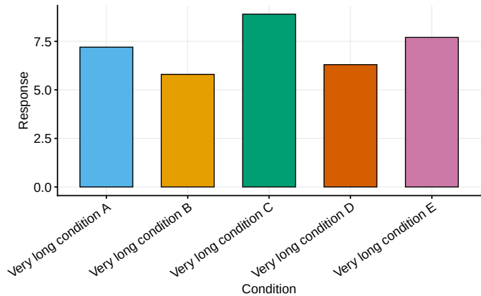
Long category labels
