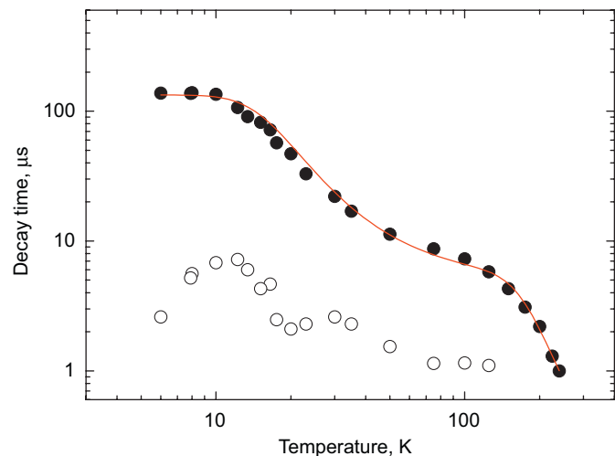
Fig. 3. Temperature dependence of the scintillation decay time constants of BGO (excitation with ^{241}\text{Am} \alpha -particles). Open and solid symbol represent the fast and the slow time constant, respectively, obtained from a fit with two exponential functions. The solid curve shows the best fit to the experimental data using the three-level model of emitting centre. Parameters of the fit are given in text.
