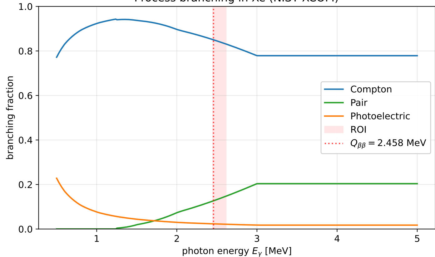
Process branching in Xe (NIST XCOM)
