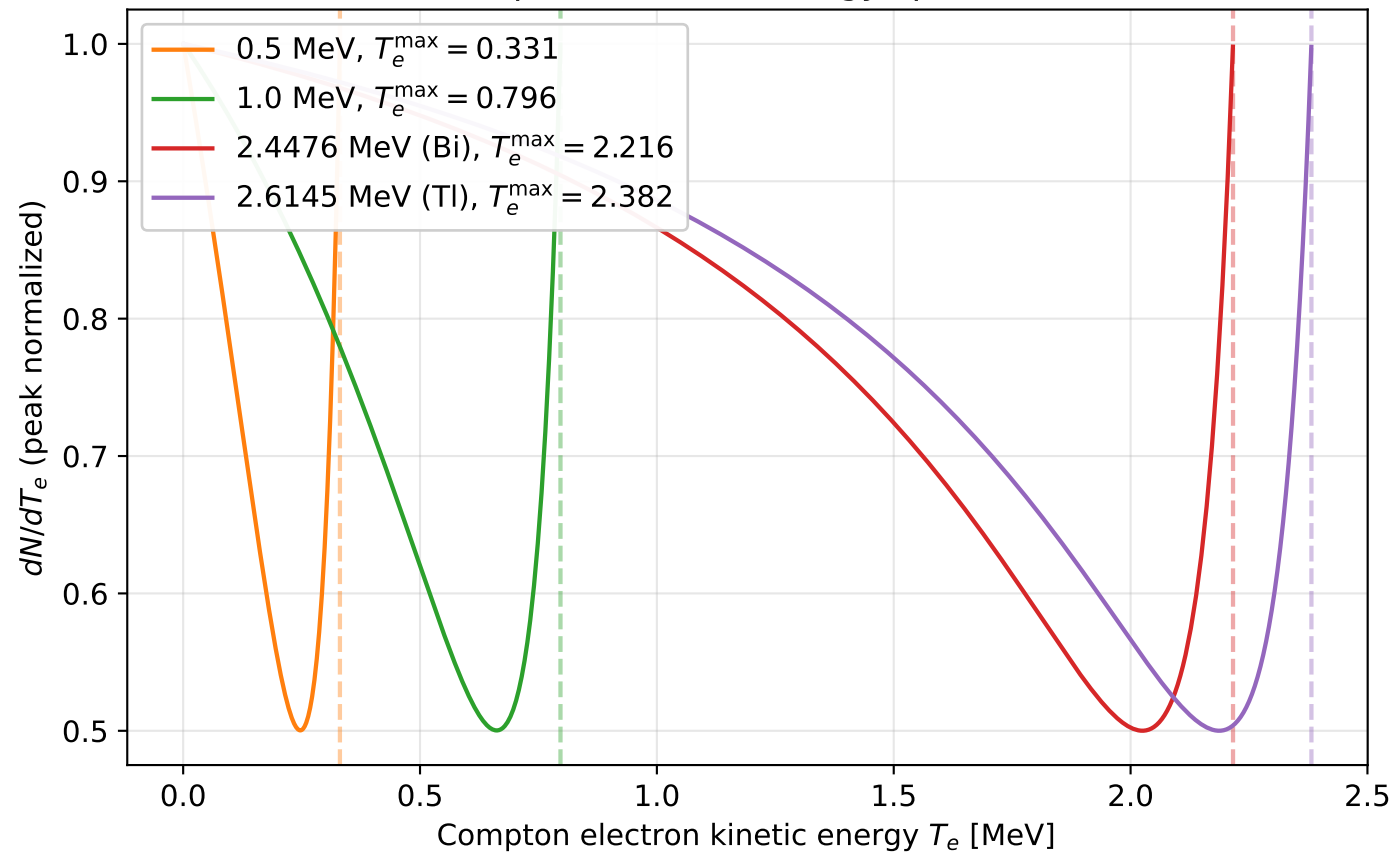
Compton electron energy spectrum
