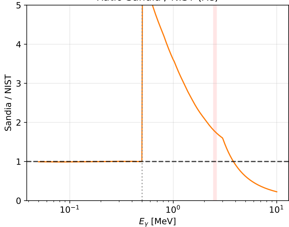
Ratio Sandia / NIST (Xe)
