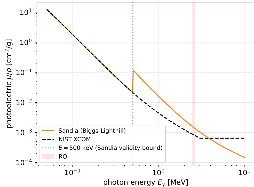
Sandia vs. NIST photoelectric in Xe
