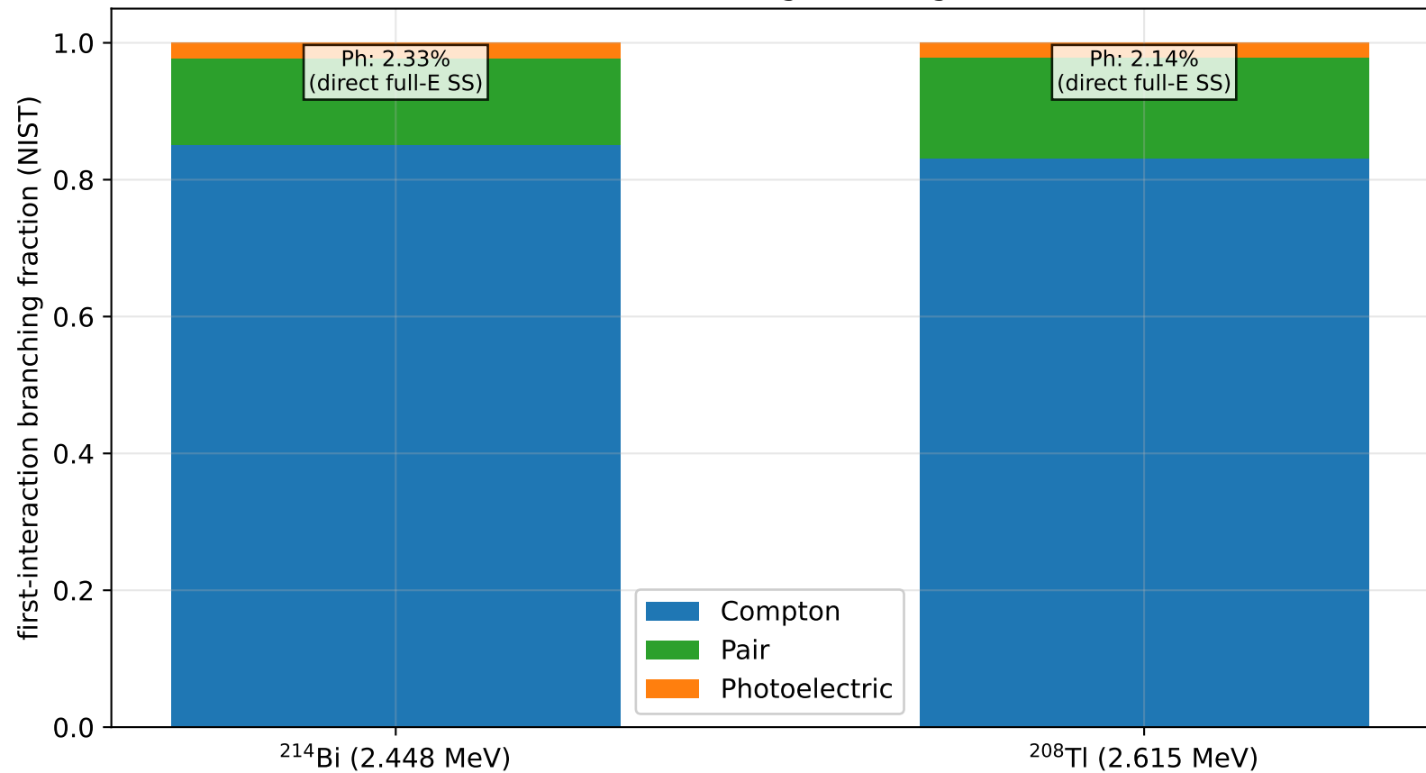
First-interaction branching for ROI gammas in Xe
