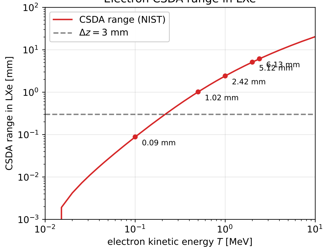
Electron CSDA range in LXe
