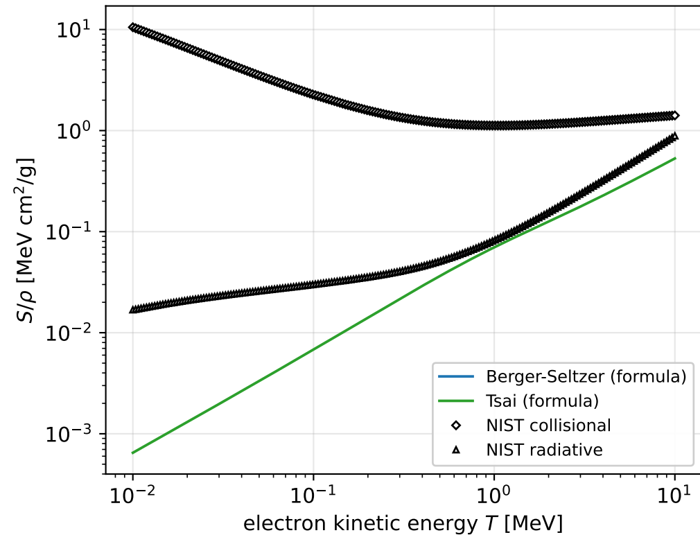
Electron stopping power in Xe
