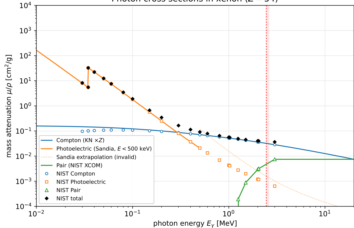
Photon cross sections in xenon ( Z = 54 )
