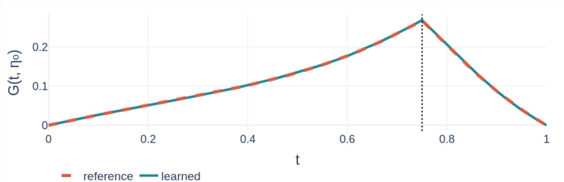
FIXED- \eta SLICE, \eta=0.75
