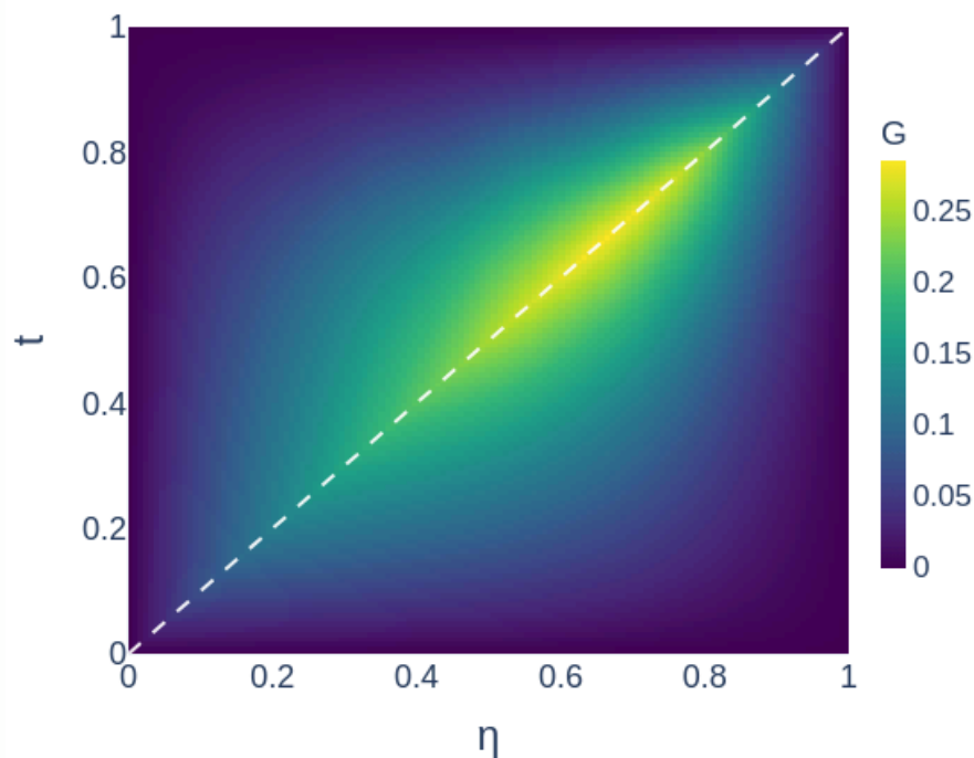
LEARNED KERNEL
