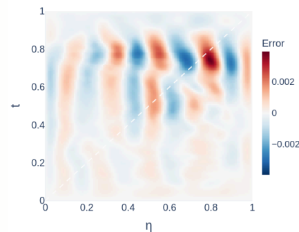
SIGNED ERROR
