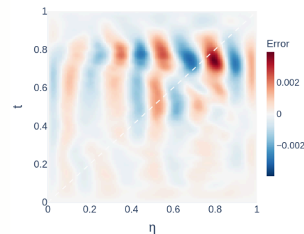
SIGNED ERROR
