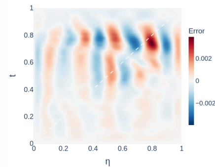
SIGNED ERROR
