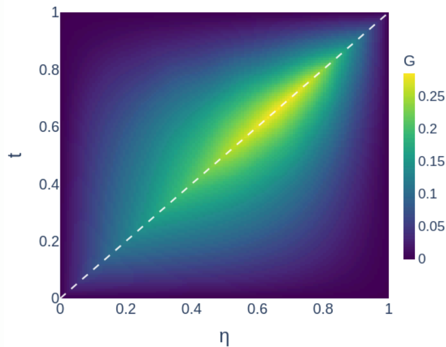
LEARNED KERNEL
