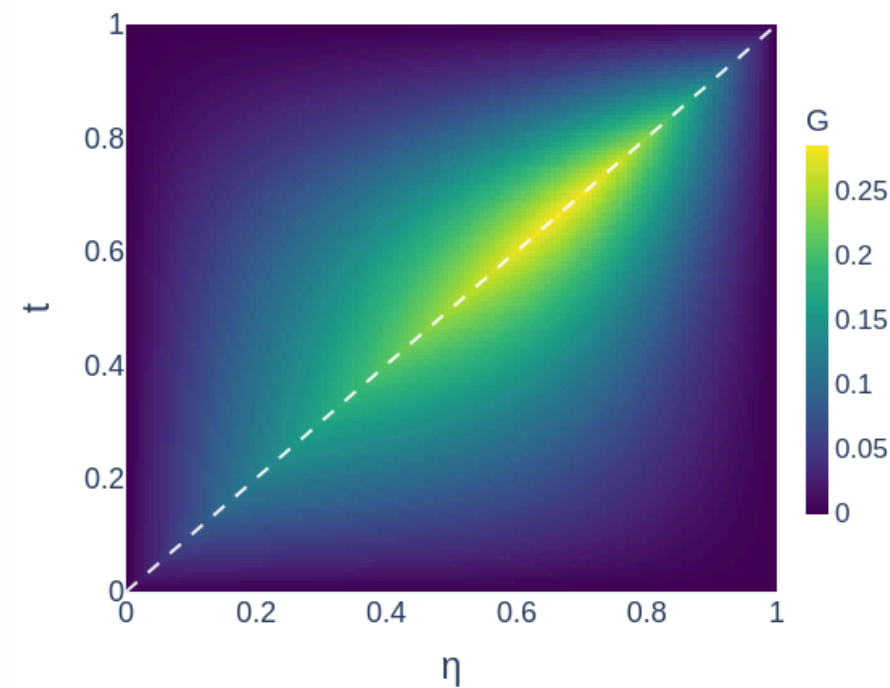
REFERENCE KERNEL
