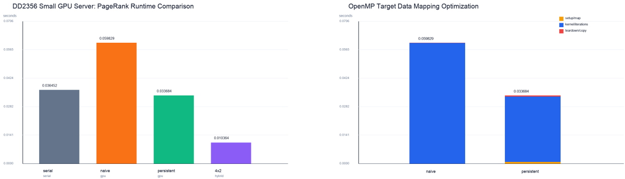
Figure 9: Same-server GPU and Hybrid timing comparison (left), and OpenMP target mapping optimization breakdown (right).
