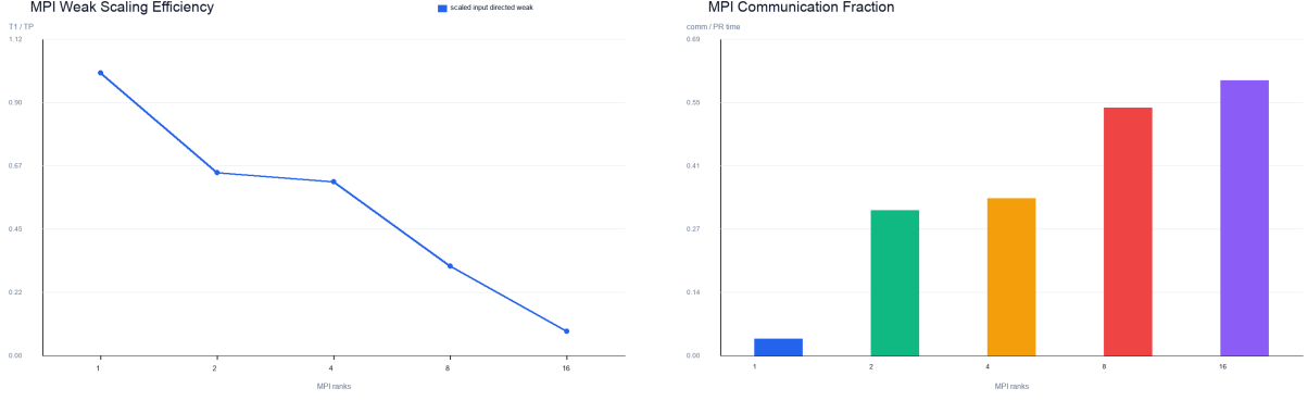
Figure 4: Dardel two-node weak-scaling efficiency and communication fraction.
