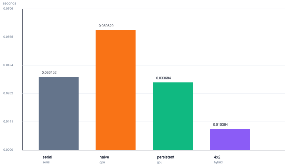
DD2356 Small GPU Server: PageRank Runtime Comparison
