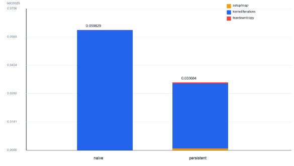
OpenMP Target Data Mapping Optimization
