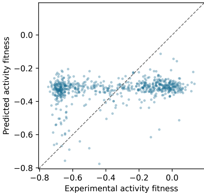
Frozen ESM-2 Test Spearman = 0.201
