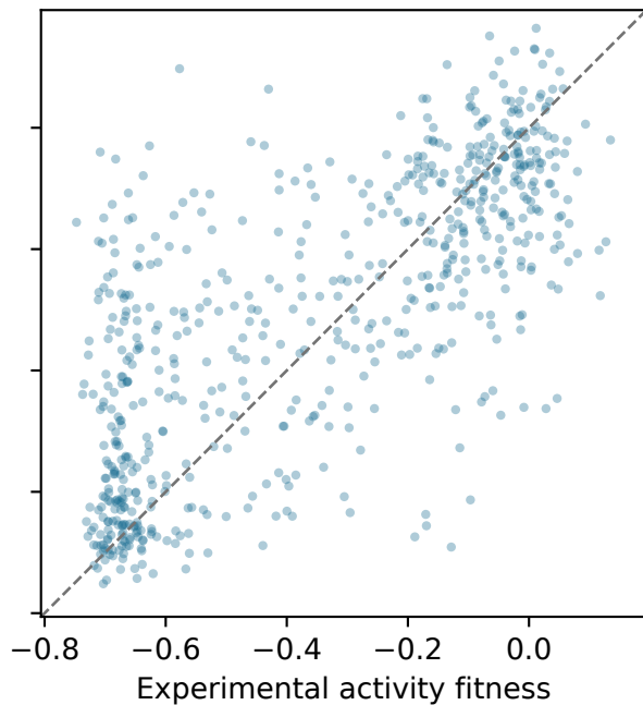
Fine-tuned ESM-2 Test Spearman = 0.716
