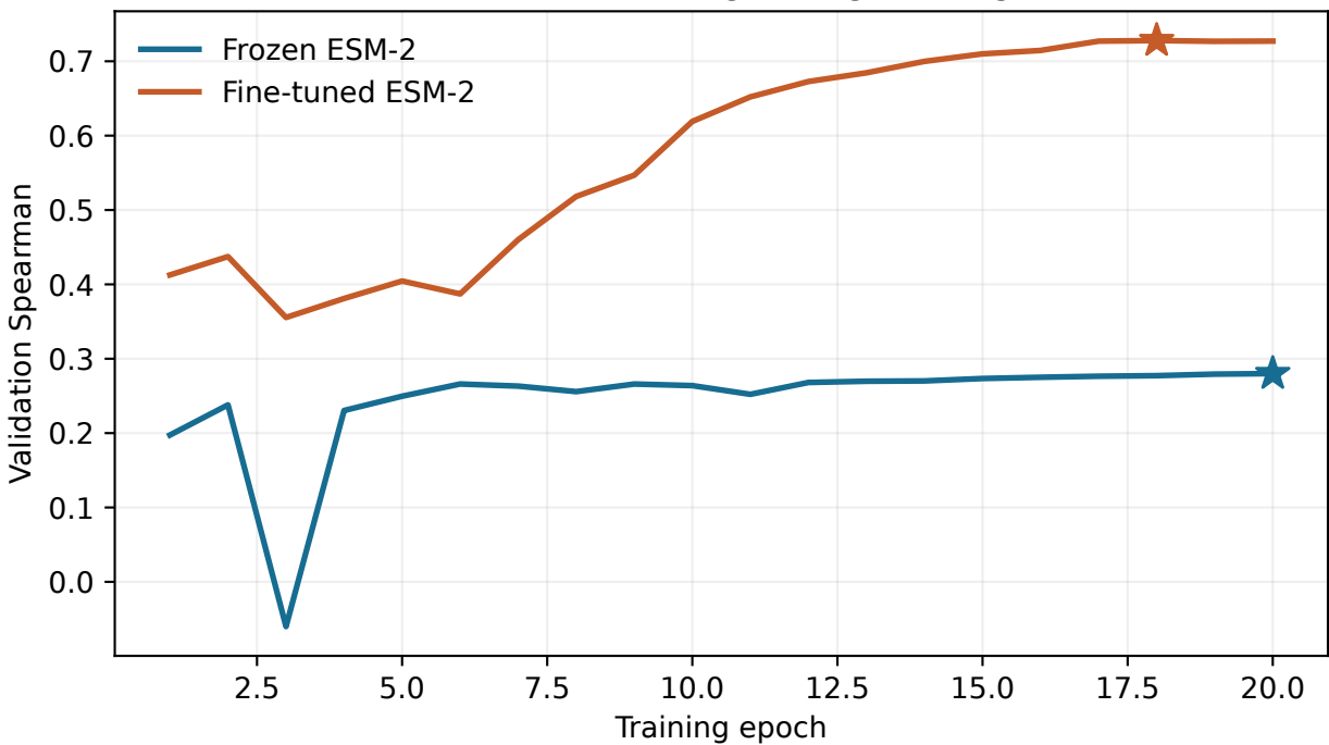
Validation ranking during training
