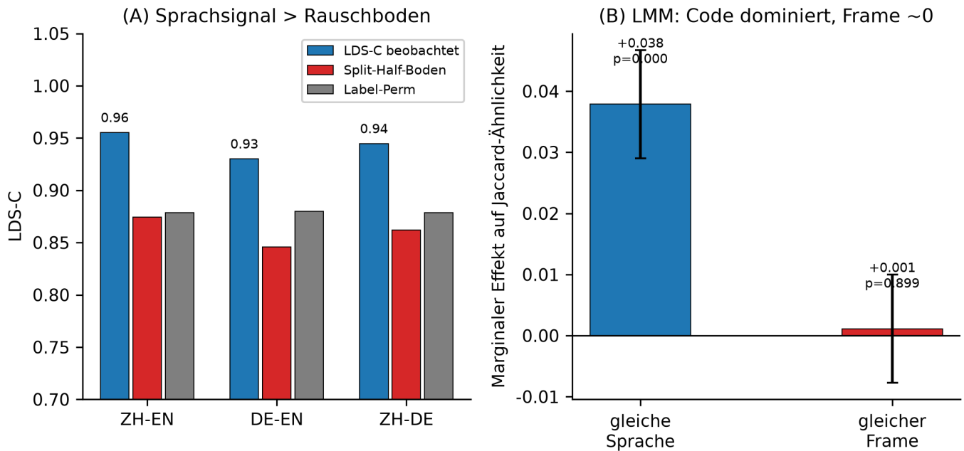
Abb. 13 — Mechanismus (P1/LMM). (A) Signal Boden (Split-Half + Label-Perm); (B) LMM: Code +0,038 ( p < 0,001 ), Rahmen +0,001 ( p = 0,90 ). Single-model Within-Subject, s. § 5.6.
