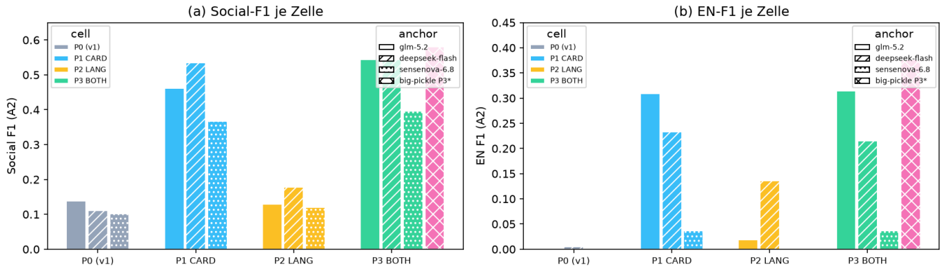
Fig v2-cells — Harness v2 factor test (seed-foreign replication)
