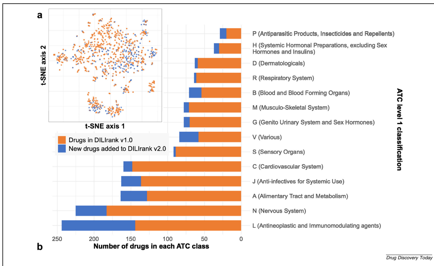
FIGURE 2 Differences between DILIRank 1.0 and 2.0: (a) Chemical space coverage of drugs, projected on a t-SNE plot; (b) Distribution of drugs by the main anatomical ATC classes in DILIRank (drugs with no ATC code are excluded from the plot).
