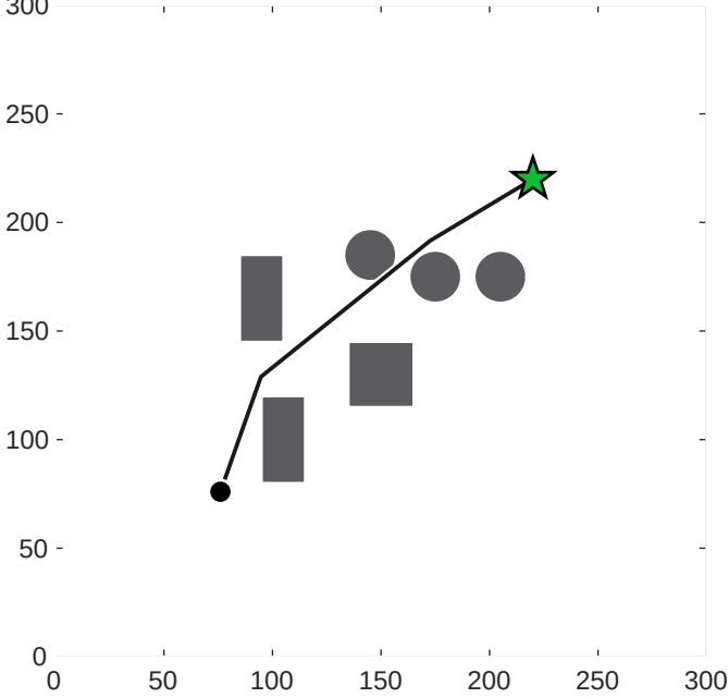
RRT-Connect | no sample set (path shown) | mean L = 213.5 (rank 6/9)
