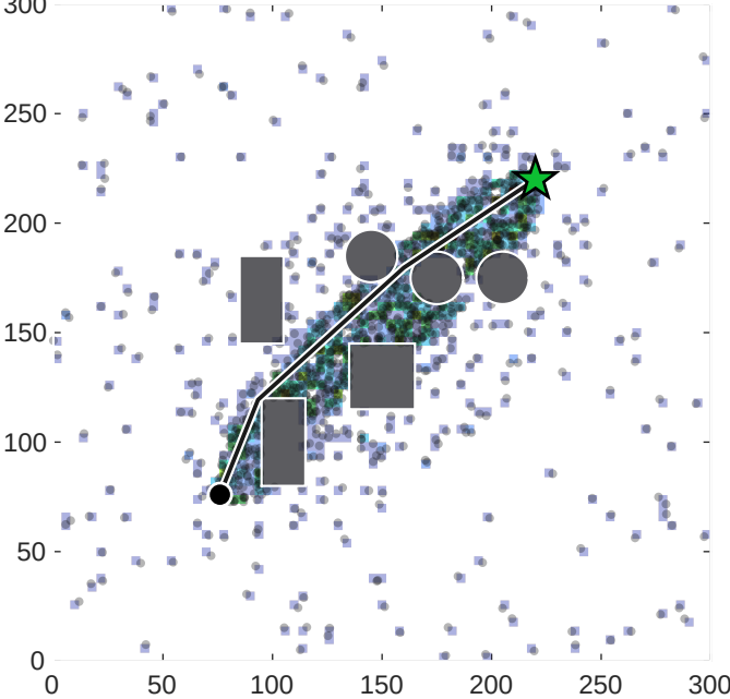
BIT* | 1315 samples | mean L = 209.4 (rank 1/9)
