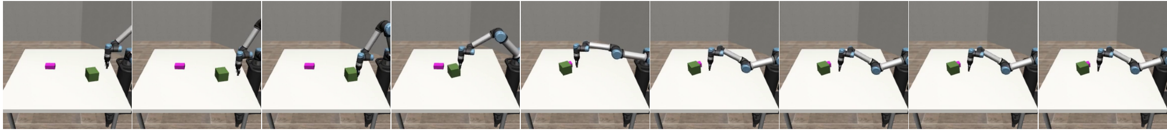
Behavior Cloning
