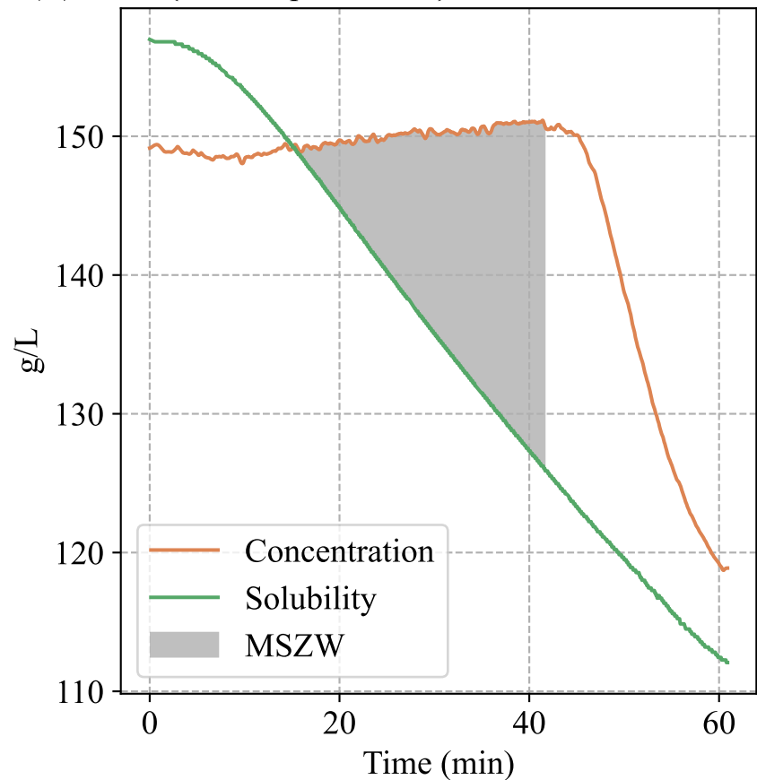
(E) 0.3 \text{ }^\circ\text{C}/\text{min} - Concentration vs Solubility
