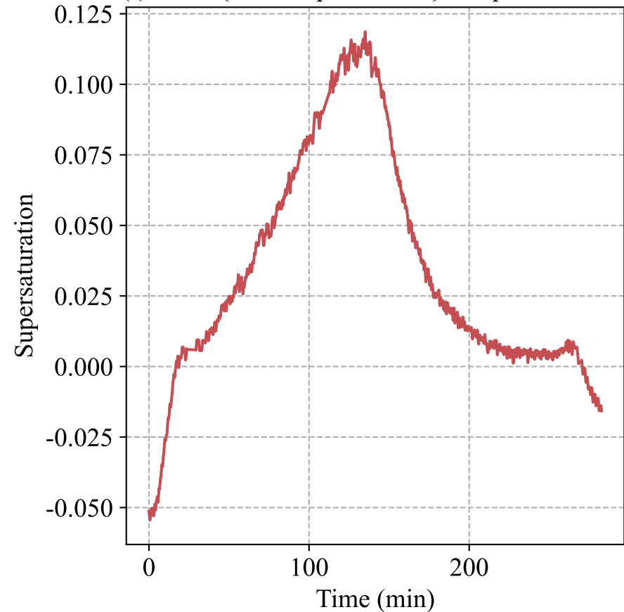
(I) 0.1 \text{ }^\circ\text{C}/\text{min} - Supersaturation
