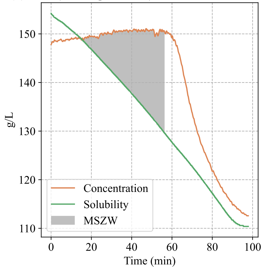
(H) 0.1 \text{ }^\circ\text{C}/\text{min} - Concentration vs Solubility
