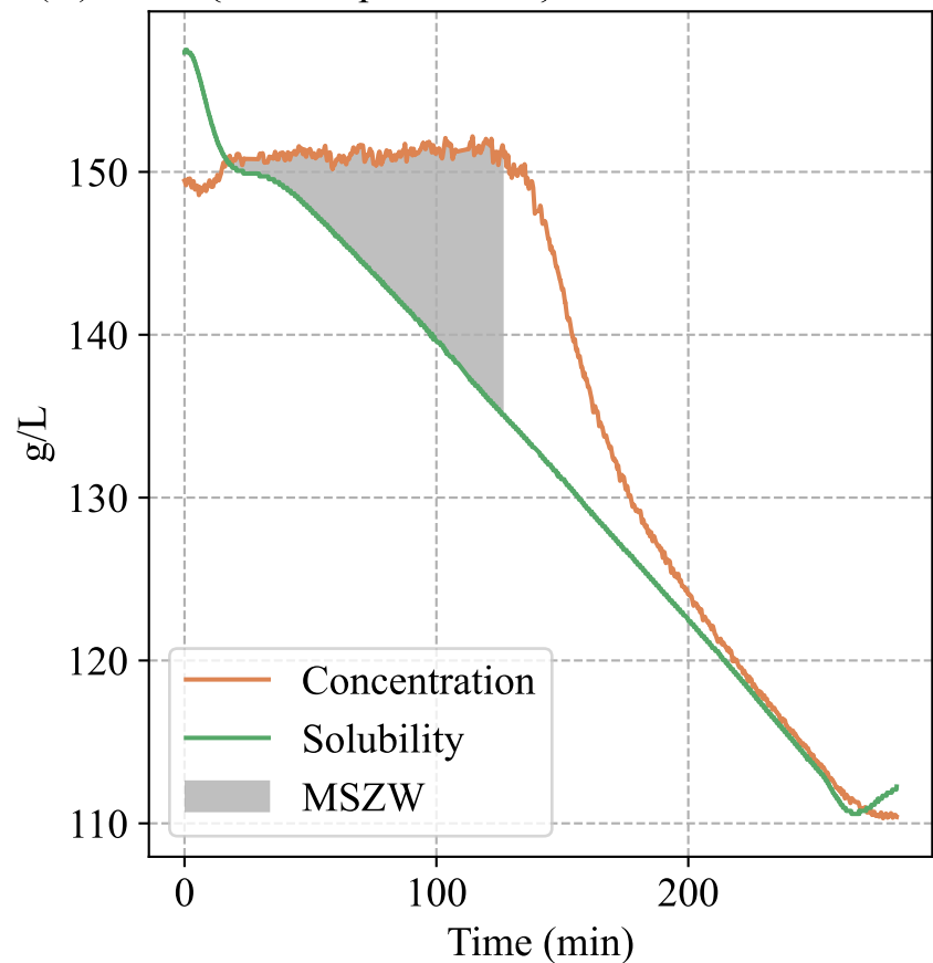
(H) 0.1 \text{ }^\circ\text{C}/\text{min} - Concentration vs Solubility
