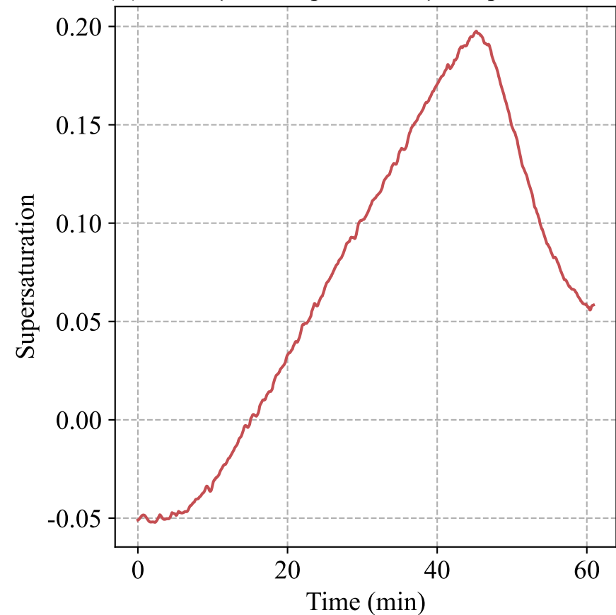
(F) 0.3 \text{ }^\circ\text{C}/\text{min} - Supersaturation
