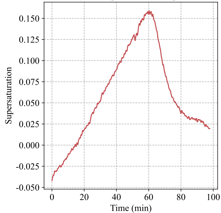
(I) 0.1 \text{ }^\circ\text{C}/\text{min} - Supersaturation
