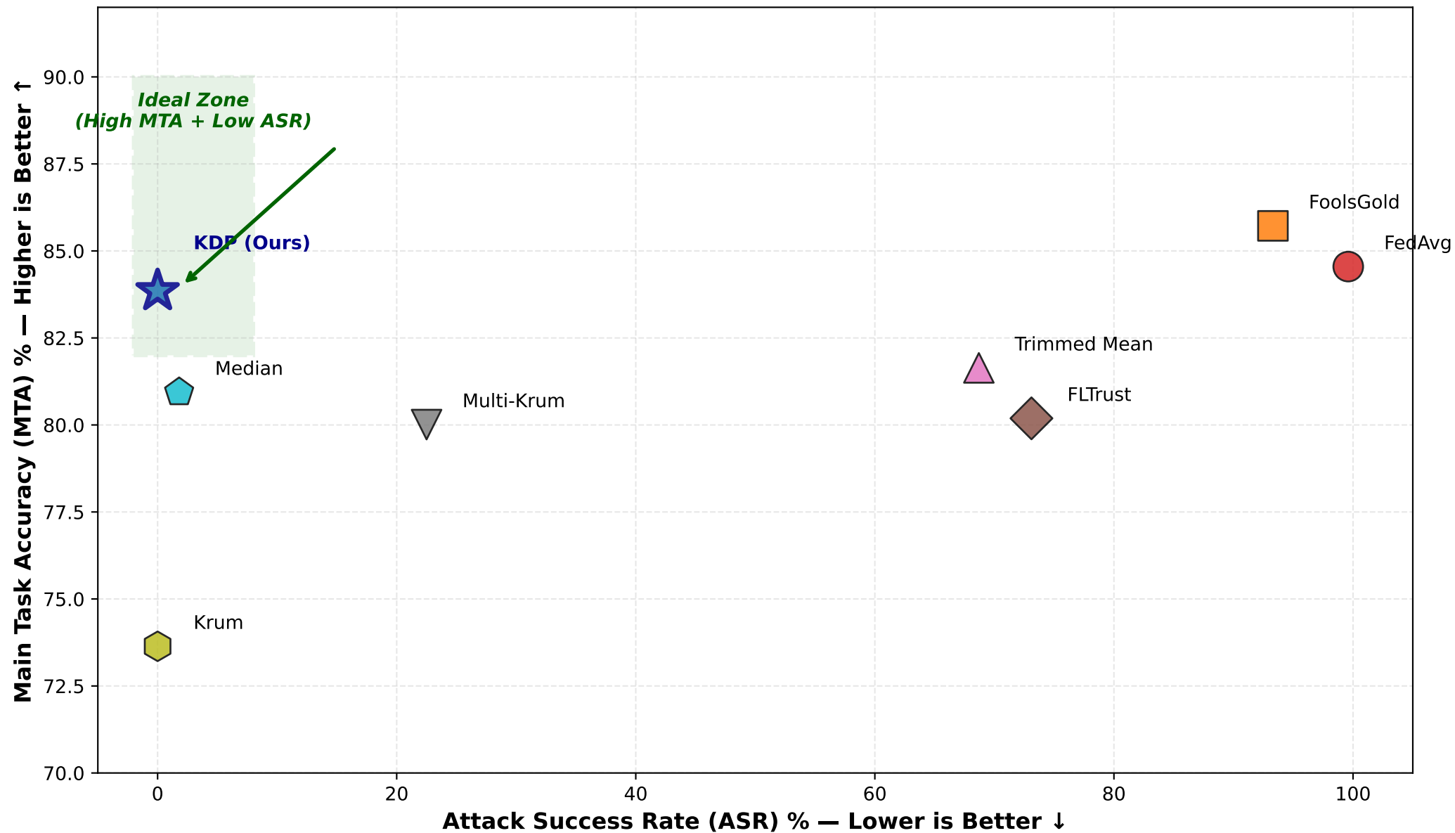
MTA vs ASR Trade-off Across Defenses (Fashion-MNIST, 20% Malicious, Backdoor Attack)
