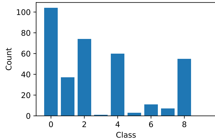
Client 0 (352 samples)
