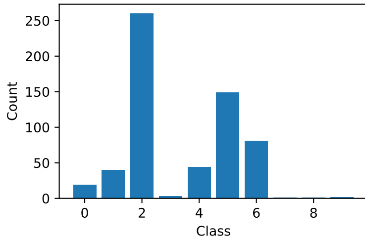
Client 1 (600 samples)
