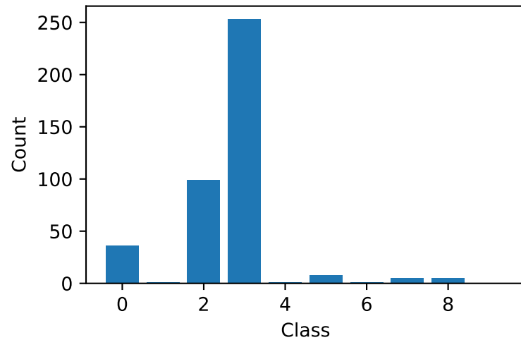
Client 2 (409 samples)
