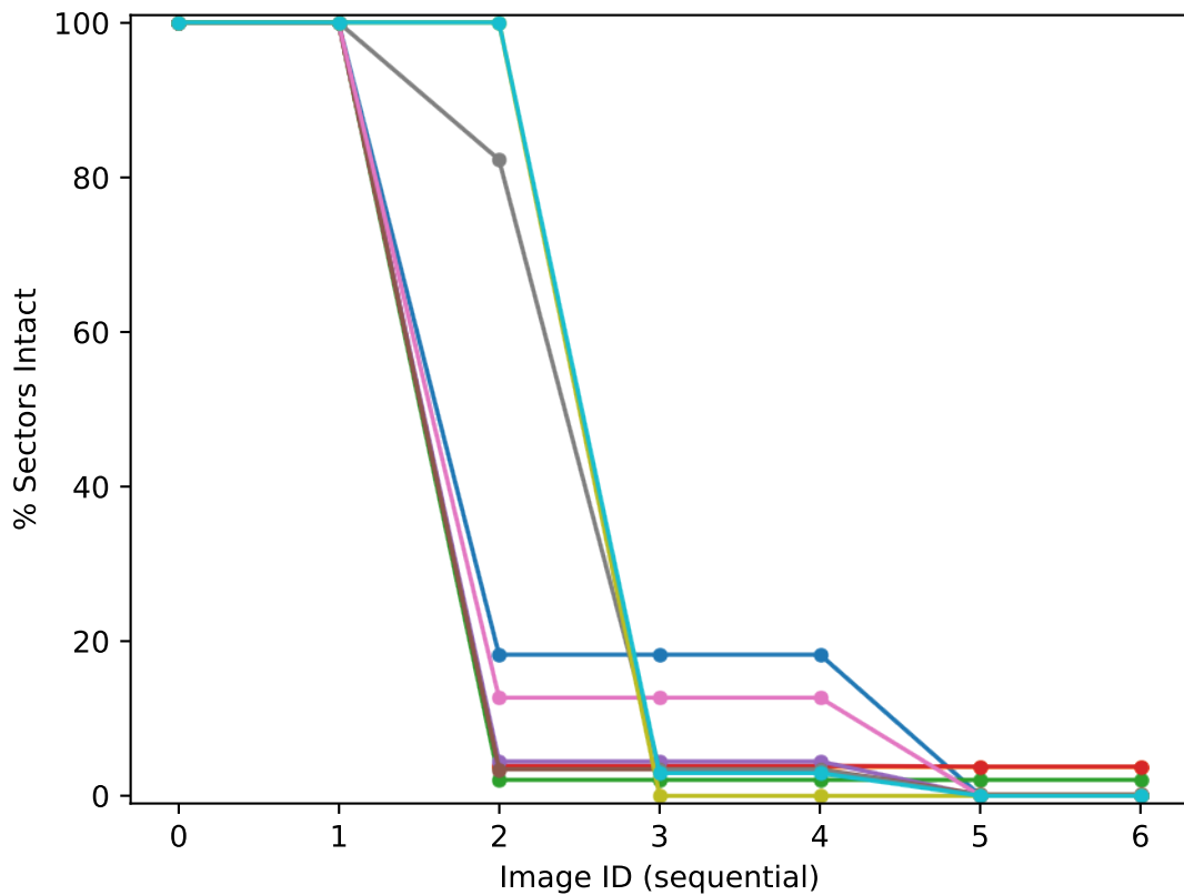
Deleted File Sector Persistence: All Files
