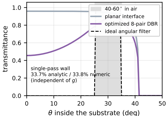
(c) single-pass angular response
