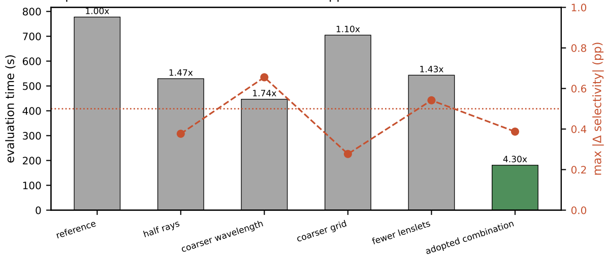
supercell cost calibration: 4.3x faster at 0.39 pp deviation
