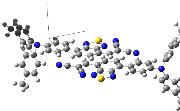
The structure of the DTDCPB chromophore dimer under investigation in this work. 2
