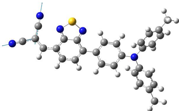
Figure 3: Structure of ground state DTD-CPB, indicating displacement vectors of nitrile stretching frequency.
