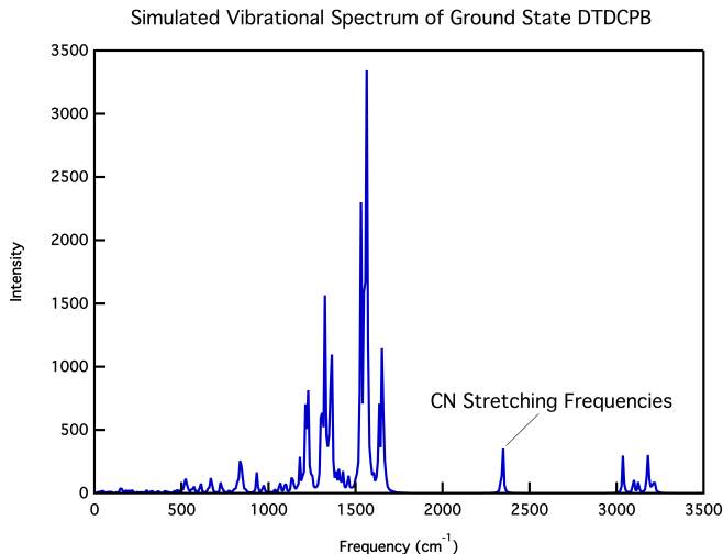
Figure 2: Ground state IR spectrum of DTDCPB.
