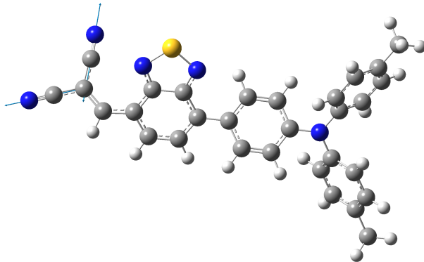
Figure 1: Structure of ground state DTDCPB, indicating displacement vectors of nitrile stretching frequency.
