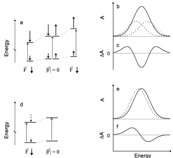
Figure 1: Illustration of the mechanism of the Stark Effect and the corresponding change in observed spectra. Level splitting due to the field is apparent in 1a (upper left), 1b (upper right) shows the corresponding first-order peak broadening, 1c (top right) is the second derivative of the ground state absorbance spectrum, and the second-order Stark effect is illustrated similarly by 1d-1f (bottom figures). 3
