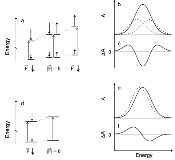
Figure 1: Illustration of the mechanism of the Stark Effect and the corresponding change in observed spectra.
