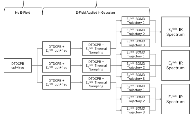
Figure 2: Diagram of the sequence of calculations for obtaining simulated spectra with BOMD. The process is identical for both the cyanide test cases and the DTDCPB monomer.
