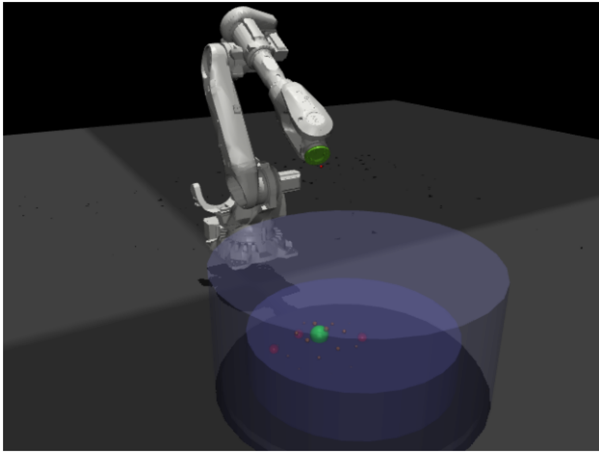
MuJoCo Thermal-Spot Coverage Environment
