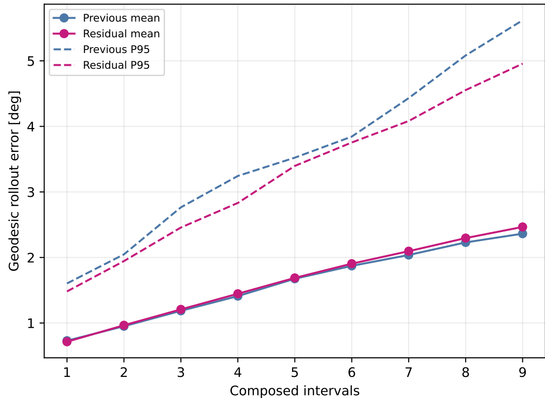
Intrinsic rollout by horizon
