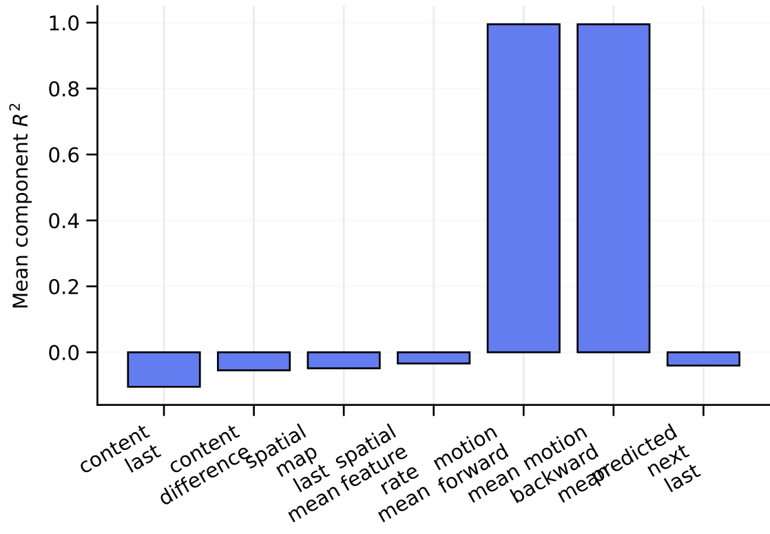
Linear angular-velocity probe
