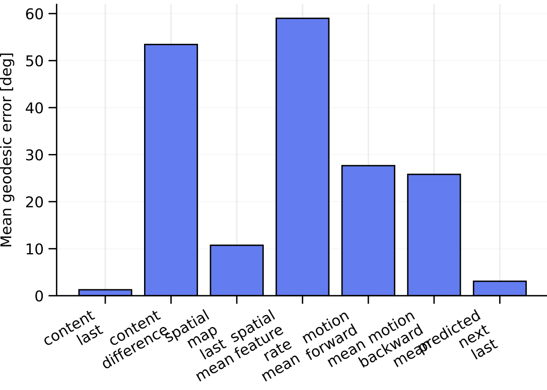
Linear orientation probe
