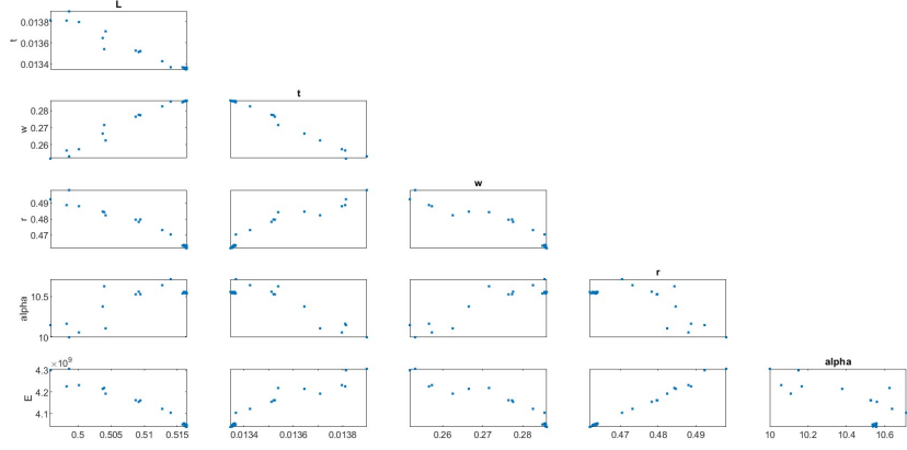
Figure 7: Model Fitting with \theta_{RED}
