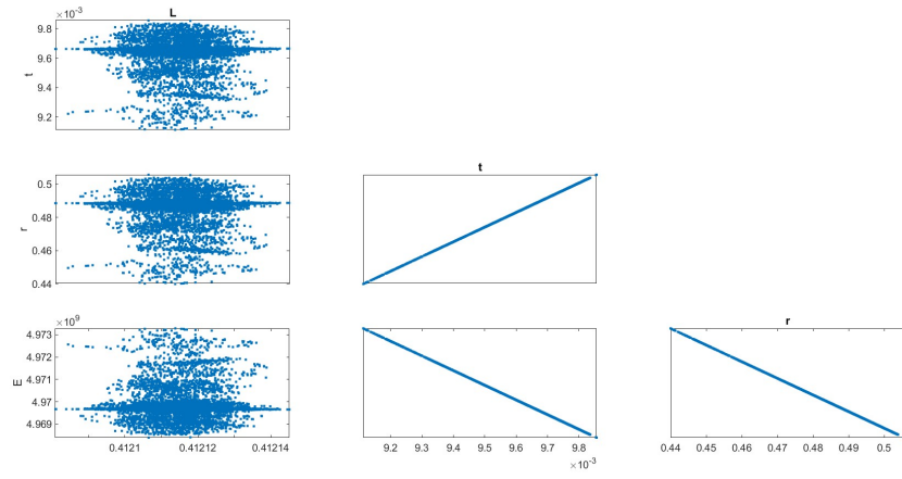
Figure 9: Model Fitting with \theta_{RED}
