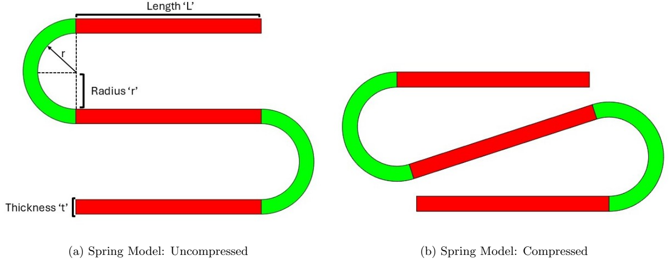
Figure 1: Spring Model Compressed and Uncompressed
