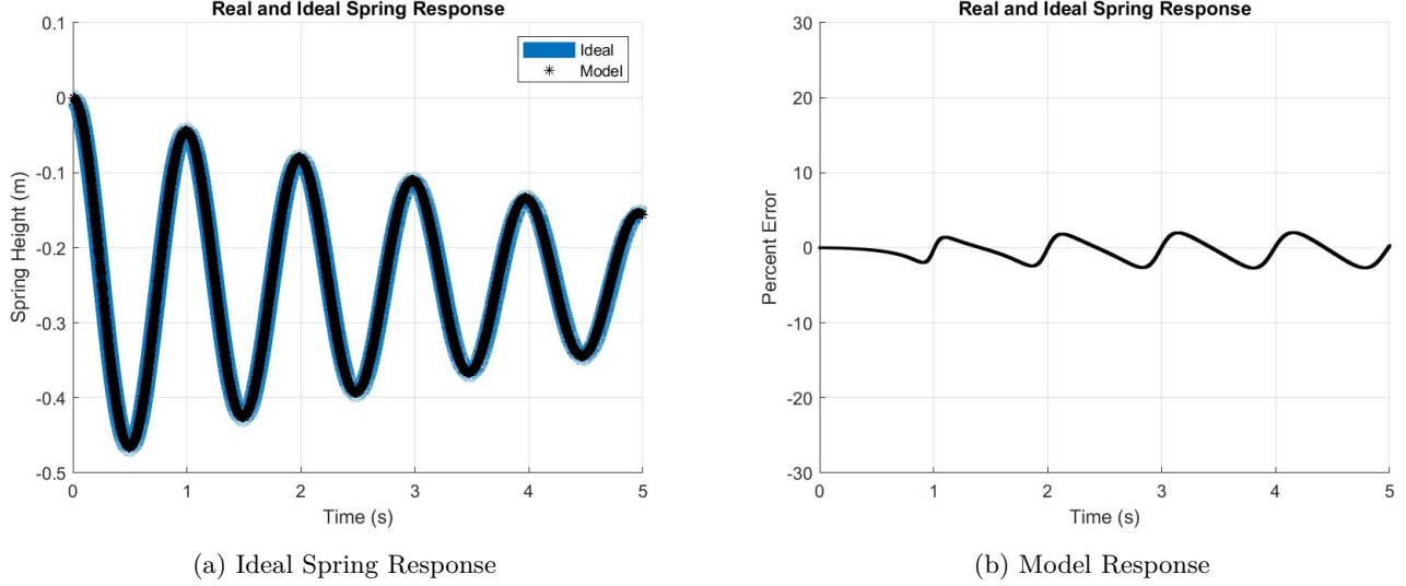
Figure 2: Ideal and Model Responses
