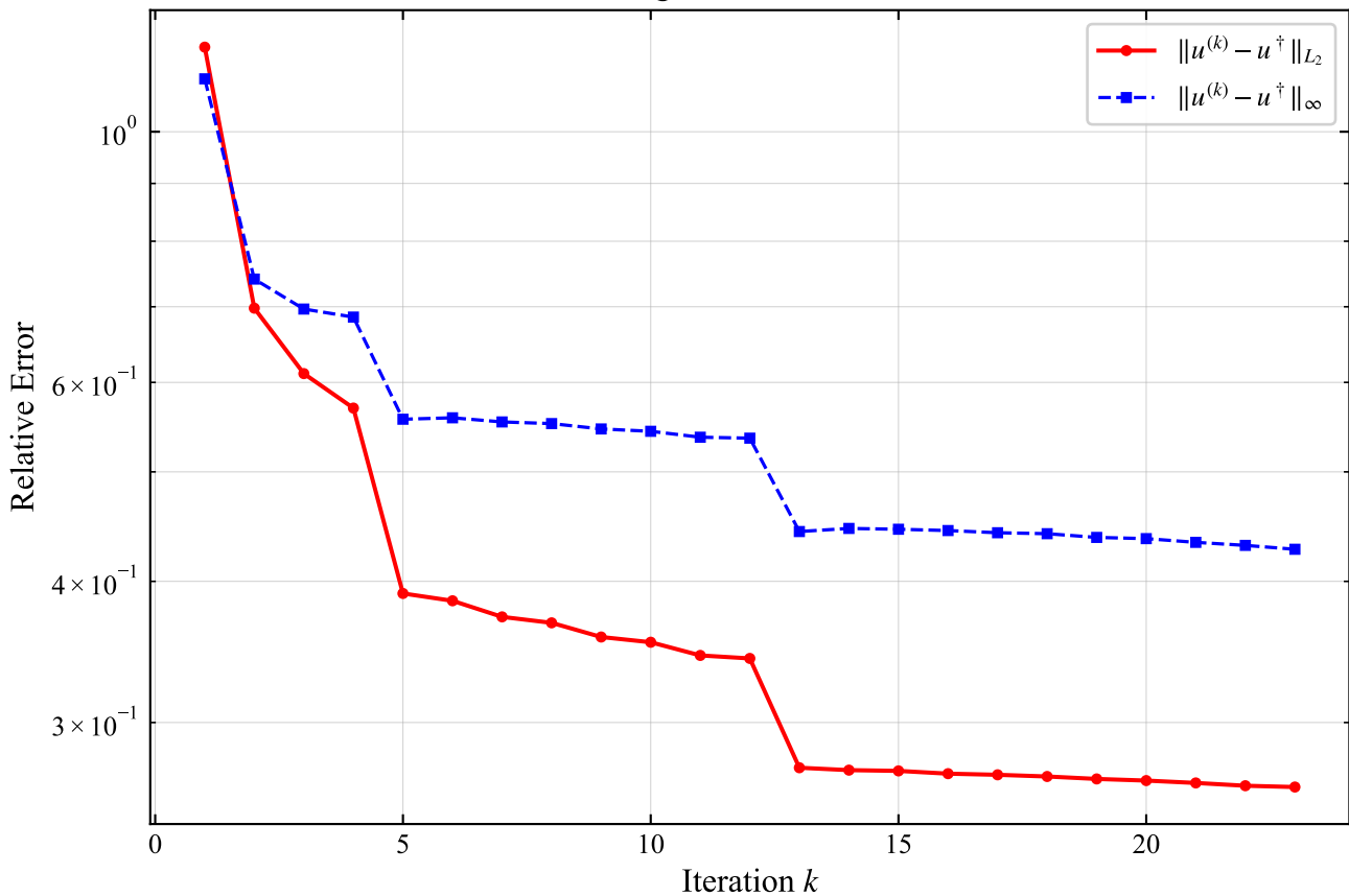
Error Convergence — GradientDescent
