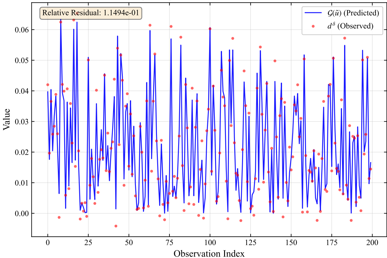
Data Fitting Comparison — NewtonCG+GradDescent
